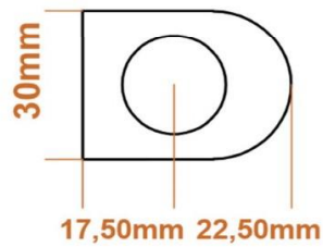
B SECTION
