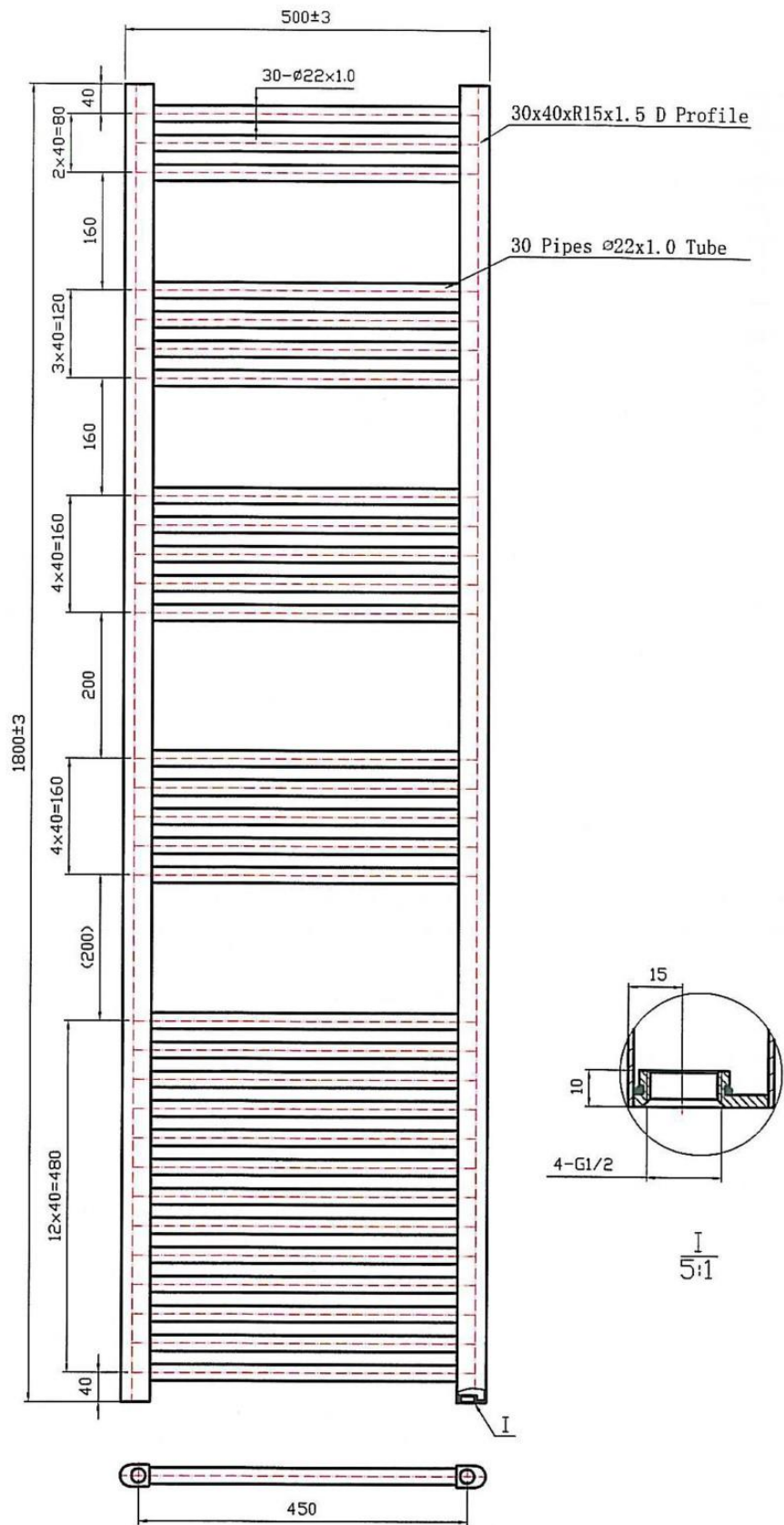
1800*500 30 pipes Straight
