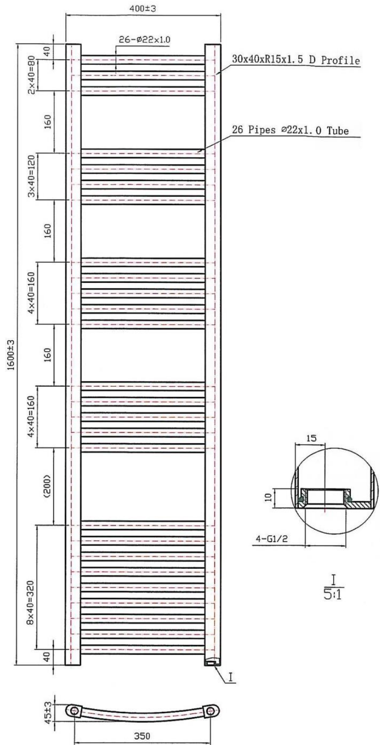
1600*400 26 pipes Curved
