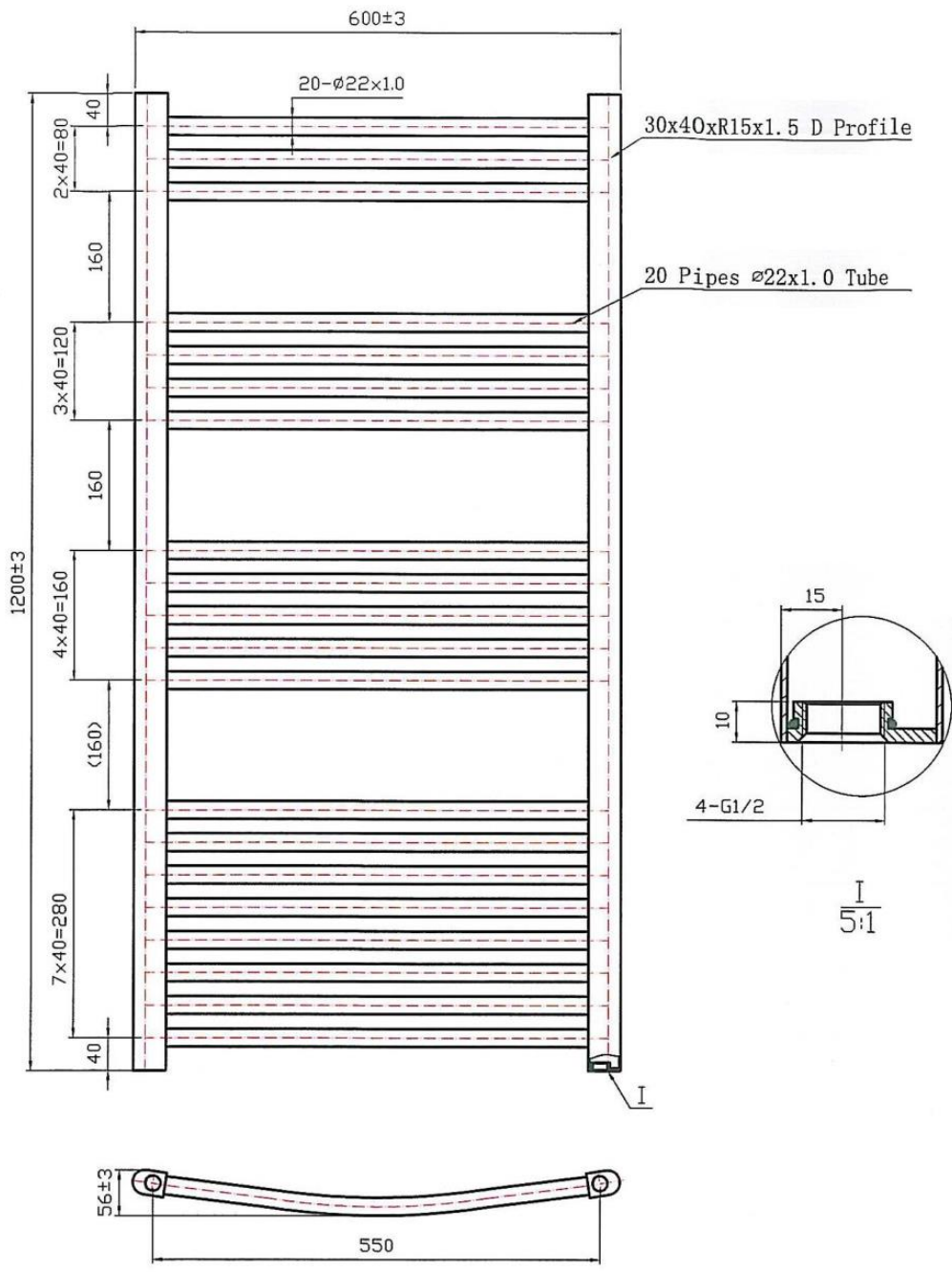
1200*600 20 pipes Curved
